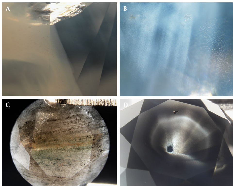
Figure 5. Cloudy regions in fancy white diamonds (top) and dark-colored particle and cloud inclusions in fancy black diamonds (bottom). Photomicrographs by Garrett McElhenny (A) and GIA staff (B–D); fields of view 2.3 mm (A), 1.6 mm (B), 6.7 mm (C), and 6.9 mm (D).
