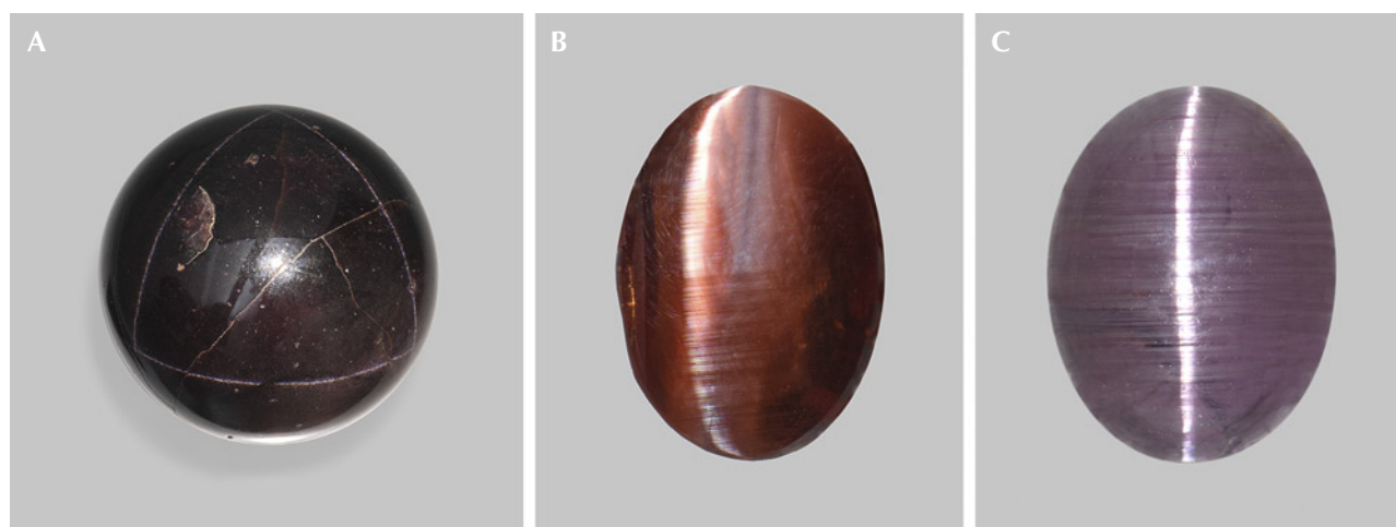
Figure 15. A: A 1,185 ct garnet sphere showing a star network of \langle 111 \rangle needle inclusions (see figure 14). The star network under rotation is shown in video 2. Courtesy of GIA Museum, collection no. 4068. B: A 1.47 ct cat's-eye almandine garnet. C: A 9.39 ct cat's-eye spinel from Sri Lanka; courtesy of John I. Koivula. Photos by Emily Lane (A) and Annie Haynes (B and C).
