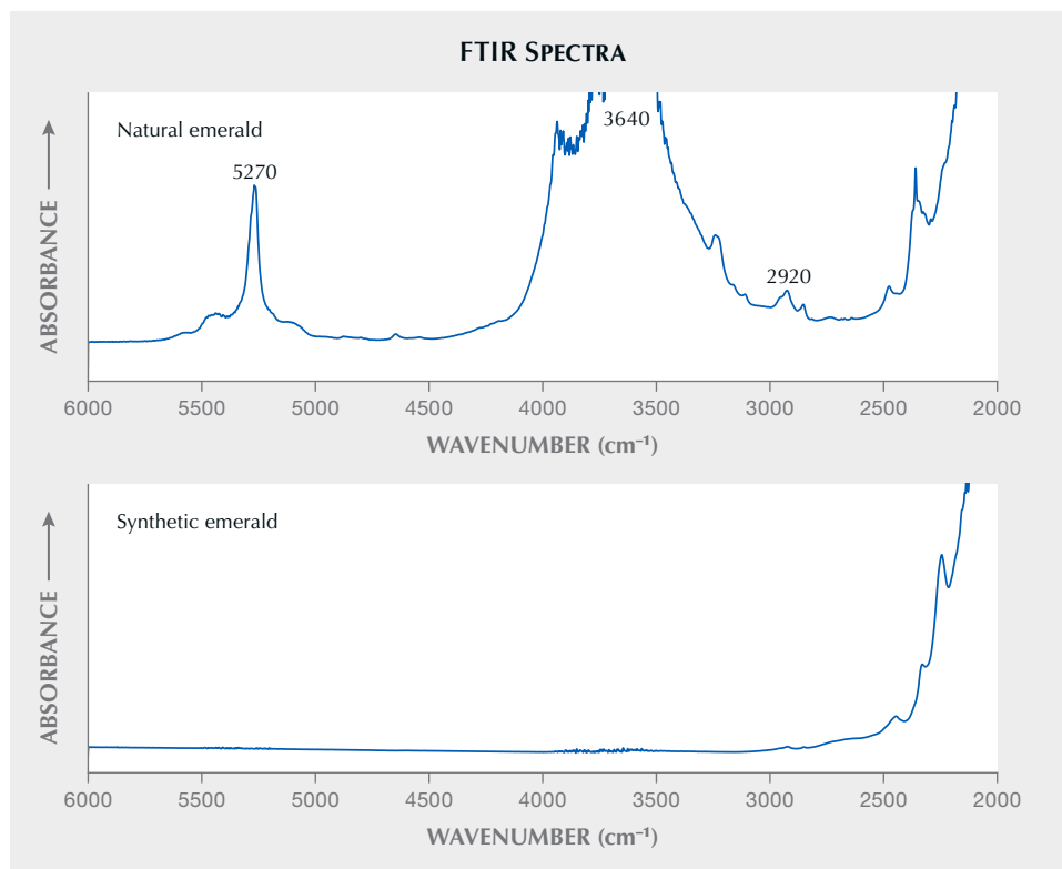
Figure 11. Typical FTIR spectra of natural emerald showing water-related features at \sim 3640 \text{cm}^{-1} (top) compared to a flux-grown synthetic emerald with no water features (bottom). The natural emerald spectrum also shows an overtone at 5270 \text{cm}^{-1} and oil peaks at \sim 2920 \text{cm}^{-1} .
