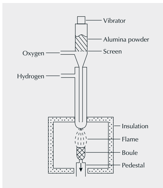
Figure 3. Drawing of a Verneuil (flame-fusion) apparatus (left) and a photo of flame-fusion crystal growth in the furnace (right). Photo courtesy of Hrand Djevahirdjian.
