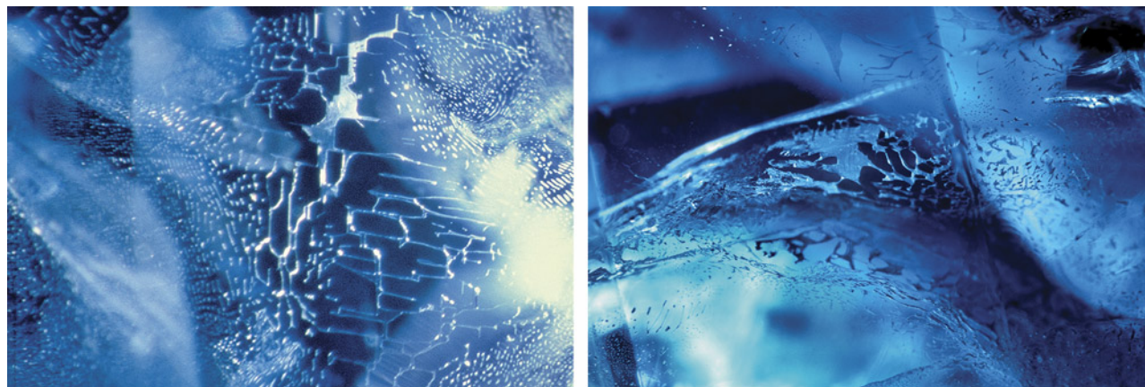
Figure 8. Images showing the similarity between fingerprints in some natural sapphires (left) and flux-healed fingerprints in some flux-grown synthetic sapphires (right), which could lead to confusion between the two. Photomicrographs by John I. Koivula.
