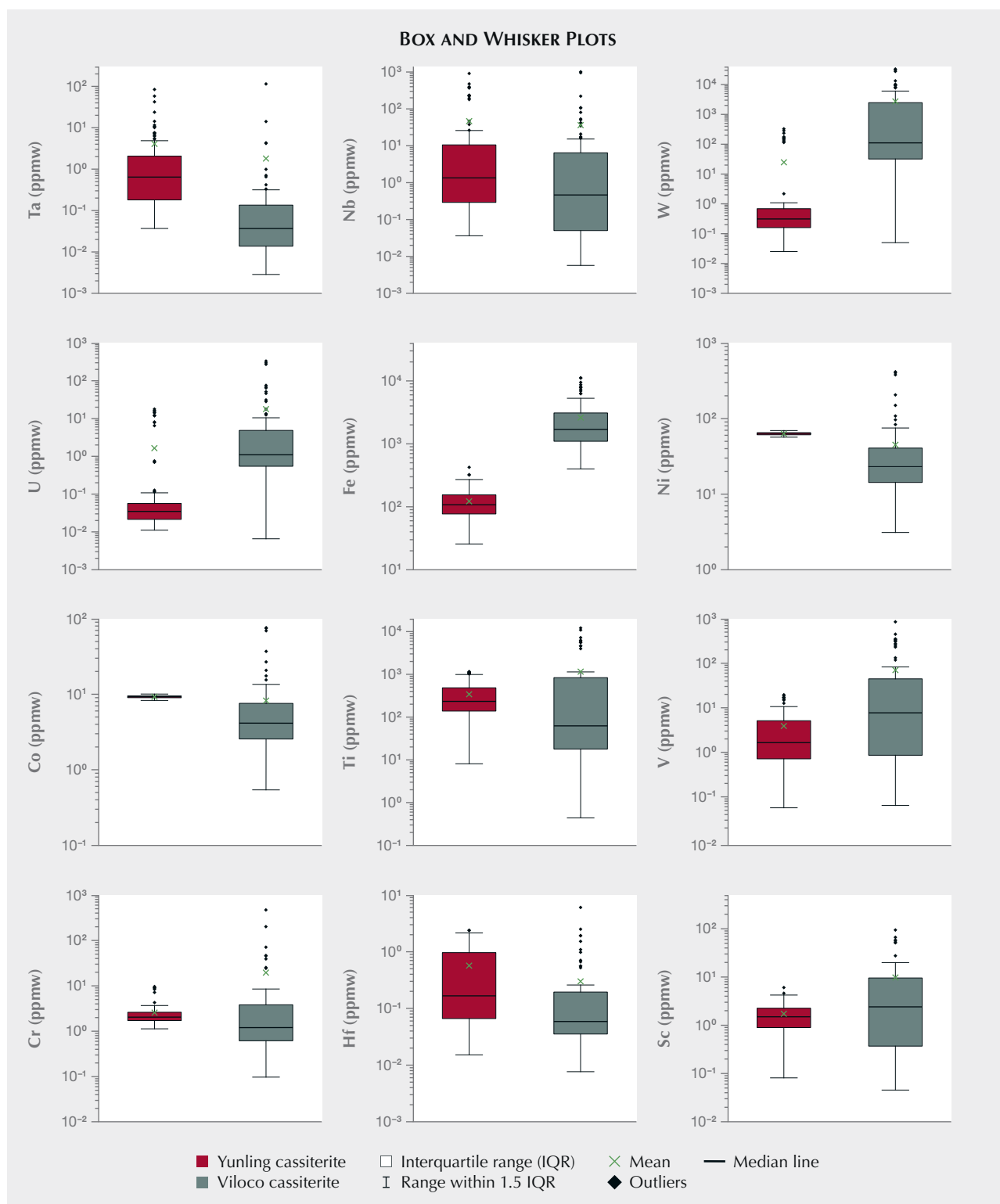
Figure 23. Selected box and whisker plots displaying trace element concentration comparisons in cassiterite from Yunling and Viloco deposits (data from Gemmrich et al., 2021). The number of analyses is 91 for Yunling and 81 for Viloco. Most elements in Viloco cassiterite (e.g., tantalum, uranium, scandium, and titanium) exhibit a wider range of spectra than those in cassiterite from Yunling. In Yunling cassiterite, the iron concentration is notably lower. Unlike Viloco cassiterite, which displays significant variations in cobalt and nickel contents, the concentrations of those elements in Yunling cassiterite remain rather consistent.
