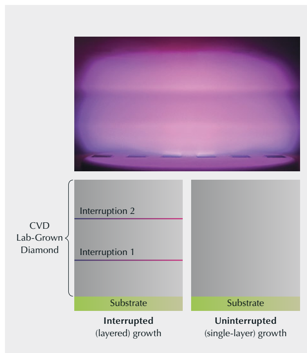
Figure 15. Top: CVD-grown diamond manufacturers grow diamond crystals using seeds (or substrates), a predetermined gas mixture, and plasma of extremely high temperature. Photo courtesy of Clarity Diamond. Bottom: Both interrupted and uninterrupted growth are applied in the industry, and each has advantages and unique challenges. Clarity Diamond uses the uninterrupted method, resulting in CVD-grown diamonds without growth lines, as displayed in this illustration.
