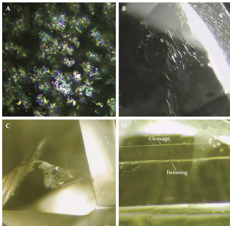
Figure 5. Inclusions in anorthoclase from south-east Vietnam. A: A myriad of incomplete thin, flat fluid inclusions reflecting interference colors (sample AF9). B: Worm-like fluid inclusions (sample AF7). C: Colorless healed fractures along the cleavage (sample AF5). D: Cleavage planes accompanied by albite-law twinning, identified using a polariscope (sample AF4). Photomicrographs by Le Ngoc Nang; fields of view 1.8 mm (A) and 2.5 mm (B–D).
