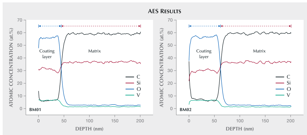
Figure 30. Corrected legends are shown for the Auger electron spectroscopy plots in figure 3 of Wu et al., “Nanoscale techniques for characterizing gemstone coatings: A case study on synthetic moissanite,” from the Spring 2024 issue.
