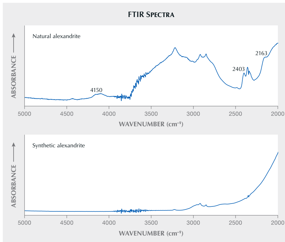
Figure 12. Typical FTIR spectra of natural alexandrite (top) showing hydrogen-related features at 2163 , 2403 , and 4150 \text{cm}^{-1} in comparison to flux-grown synthetic alexandrite (bottom), which does not have any of these features.
