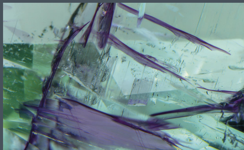
Natural radioactive fluids have infiltrated cracks in this Mozambican elbaite tourmaline, creating localized radiation-induced natural pink color zones along the walls of the fractures. Field of view 4.27 mm.
