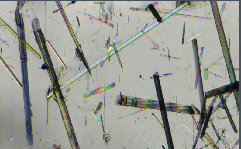
A pale blue aquamarine crystal from Pakistan contains a multitude of tourmaline inclusions that show vibrant interference colors using polarized light. Field of view 2.61 mm.
