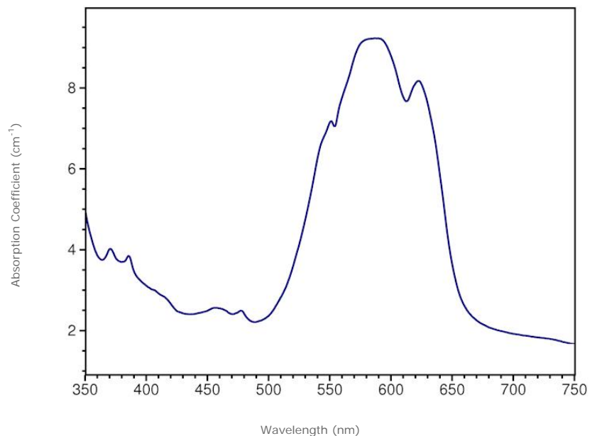
Visible Absorption | min. path length: 3.0 mm
