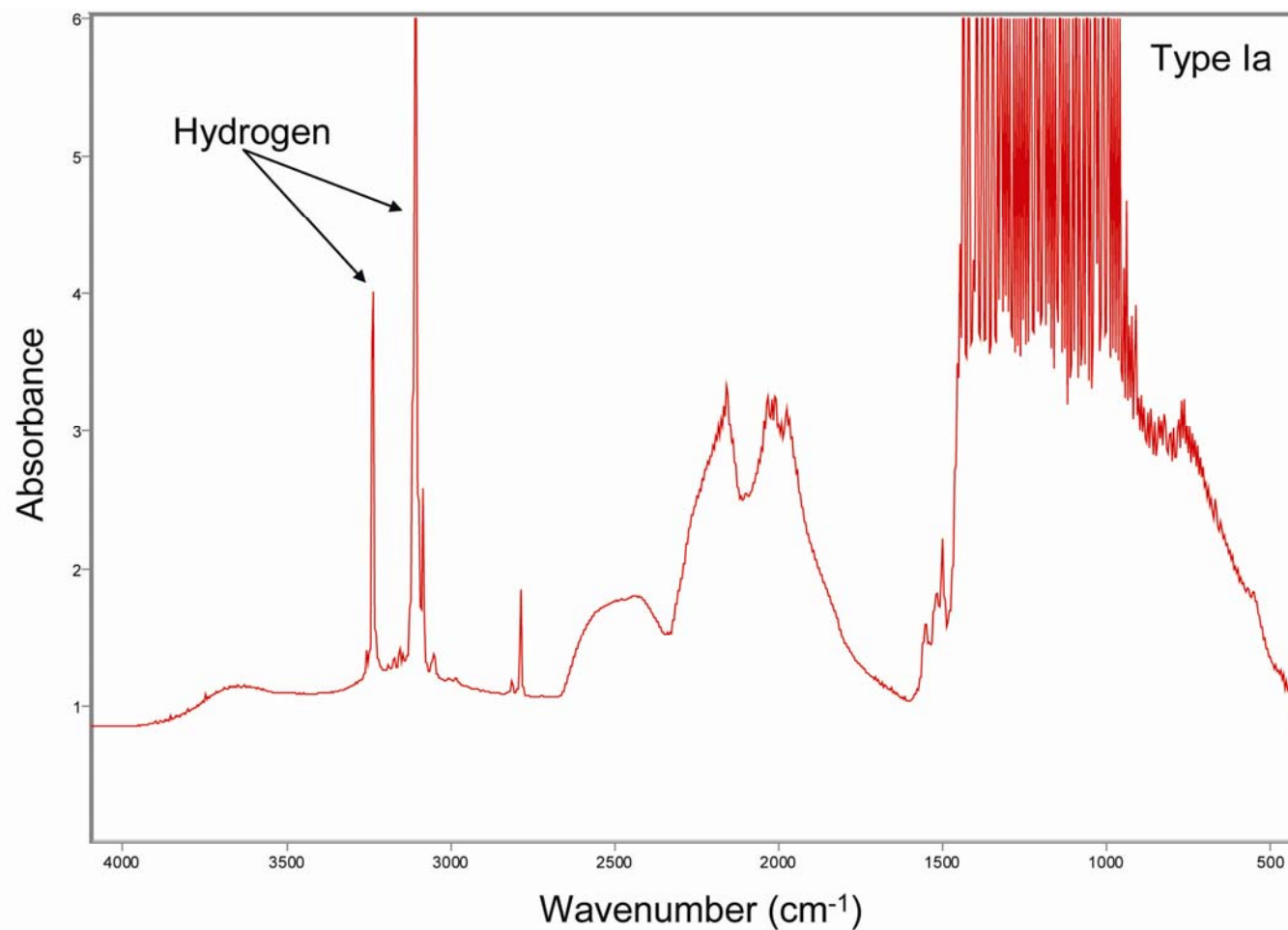
Supplemental Figure: The FTIR spectrum from the “black” diamond with deep violet bodycolor indicates that it is type Ia with abundant hydrogen impurities. Collected using Thermo Nicolet 6700 FTIR spectrometer with beam condenser and KBr beamsplitter.
