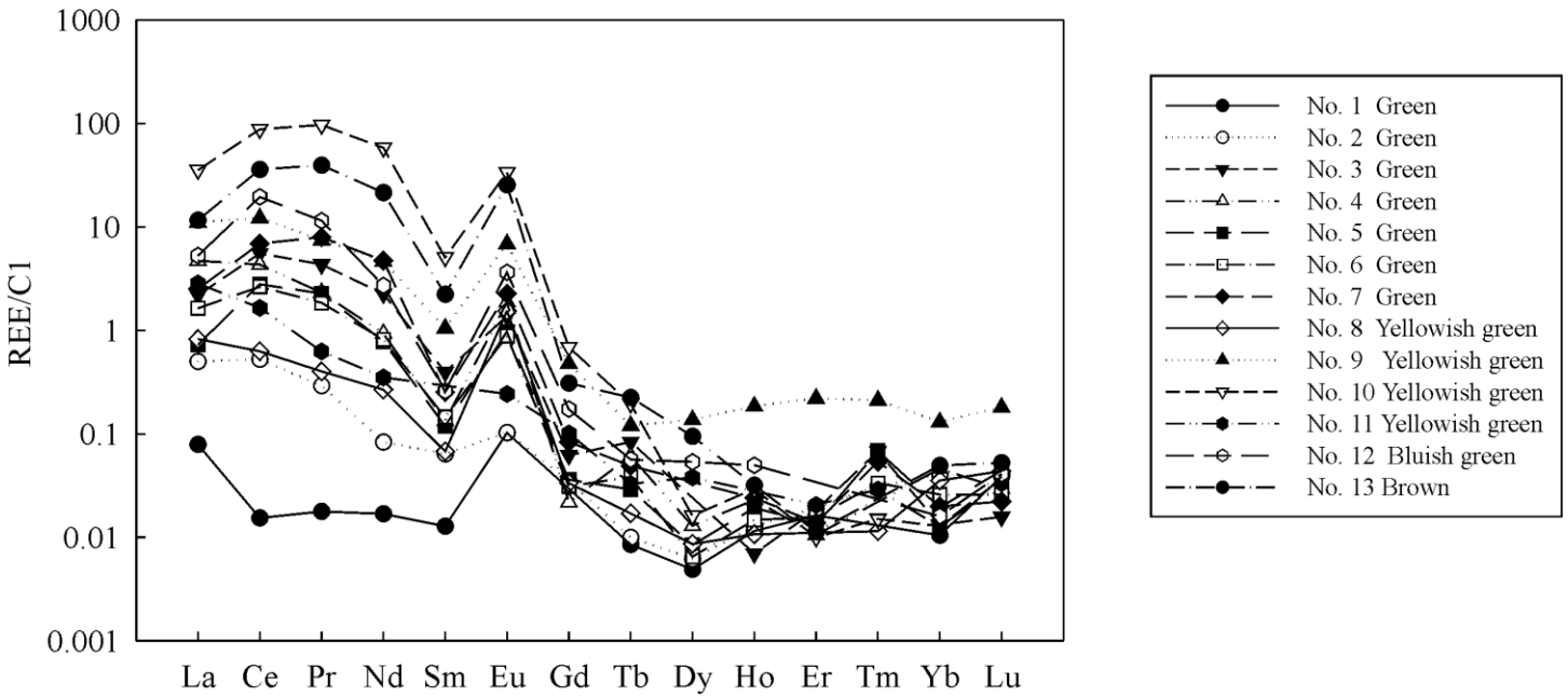
Figure DD-1. Typical of andradite, the rare-earth element composition of Antetazambato material shows enrichment in light REE and depletion of heavy REE. The data are normalized to C1 chondrite composition per standard practice.
